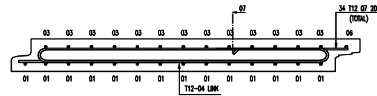
SECTION C-C
