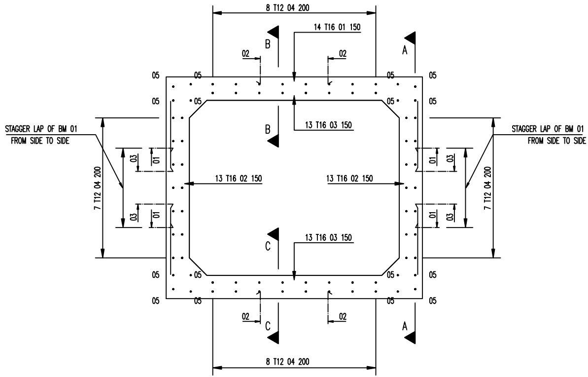
SECTION THROUGH BOX CULVERT SHOWING REINFORCEMENT
