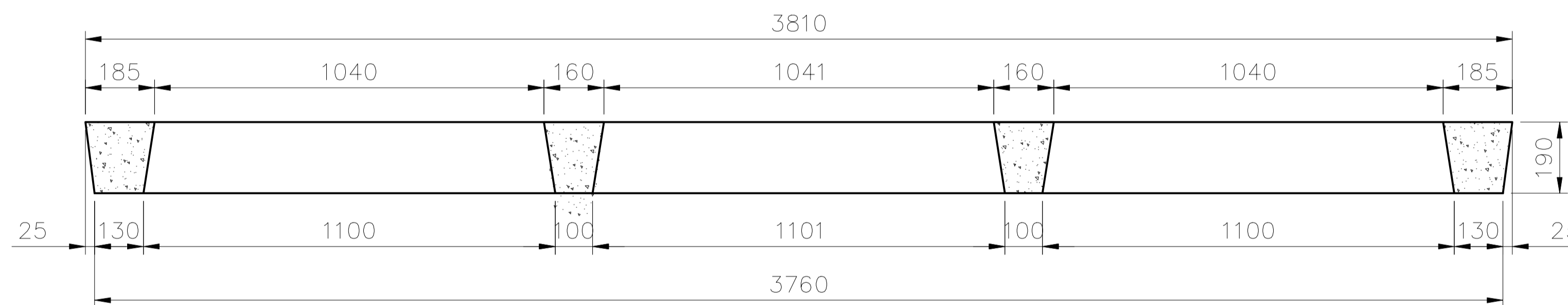
Section B-B
